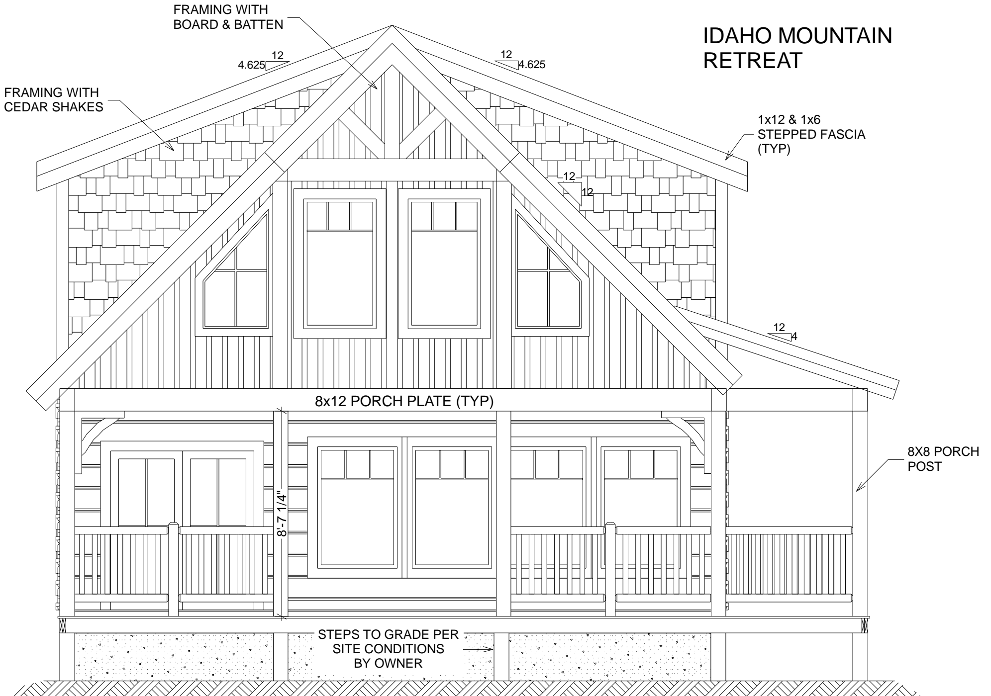
FRONT ELEVATION
