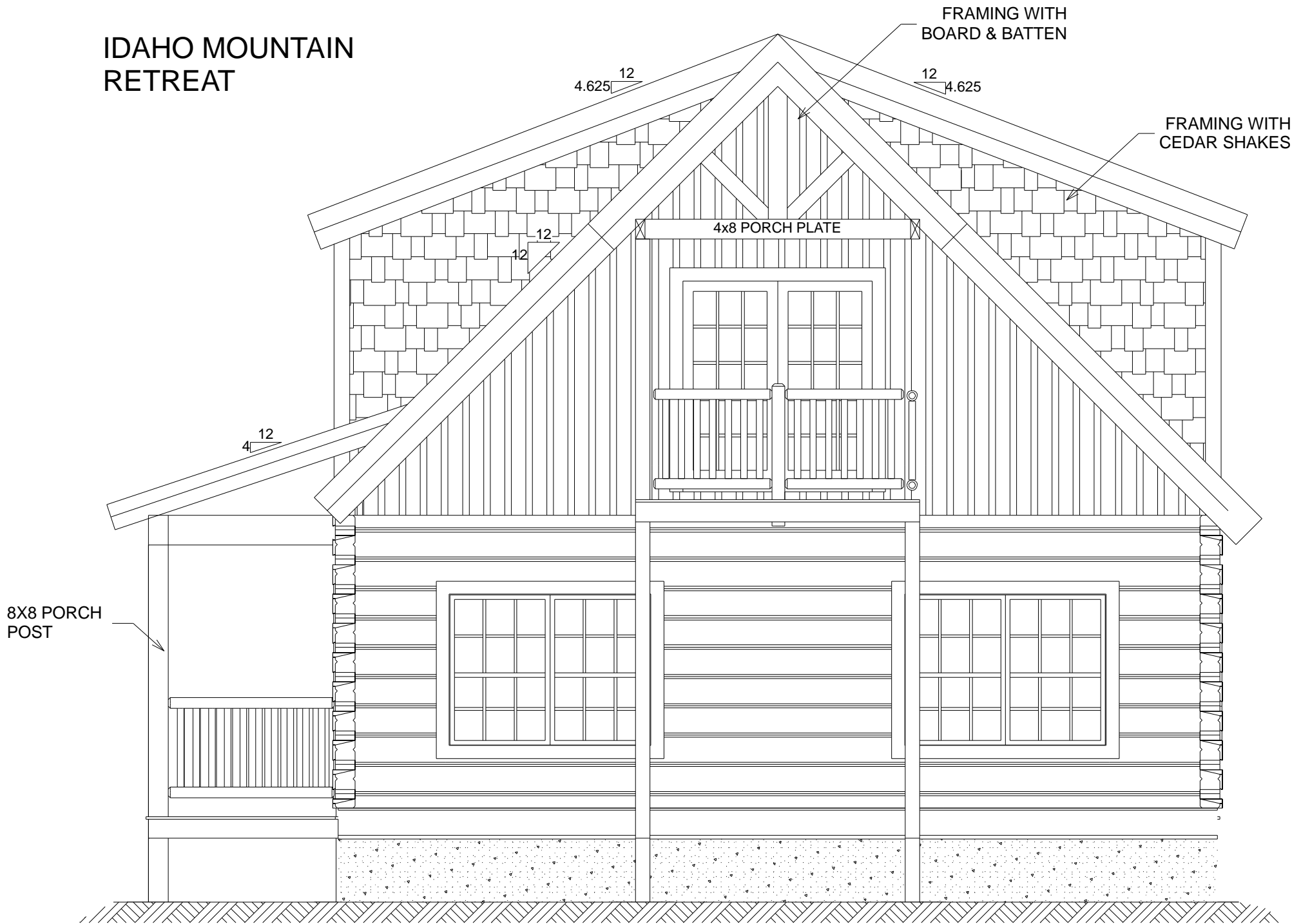
REAR ELEVATION
